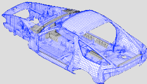
Reinforced Areas
