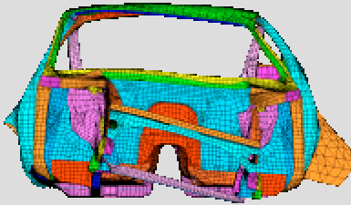
Initial Design: Low Torsional Rigidity
