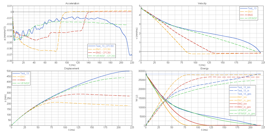
Figure 20: Comparison between test 13 and simulation
