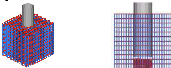
Figure 3: Characteristic deformation behaviour of T-directional locally loaded honeycomb model
