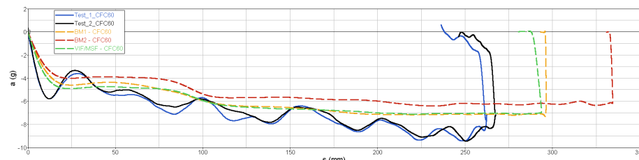
Figure 19: Comparison between test 5, 6 and simulation
