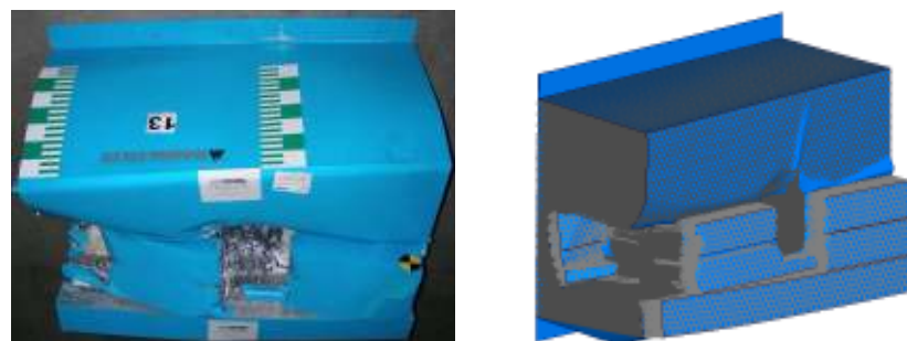
Figure 17: Deformed barriers test 13 and simulation;
